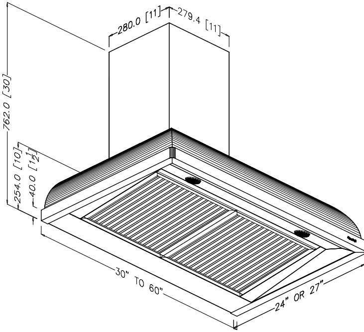
ISO VIEW
