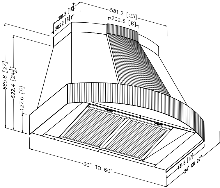
ISO VIEW
