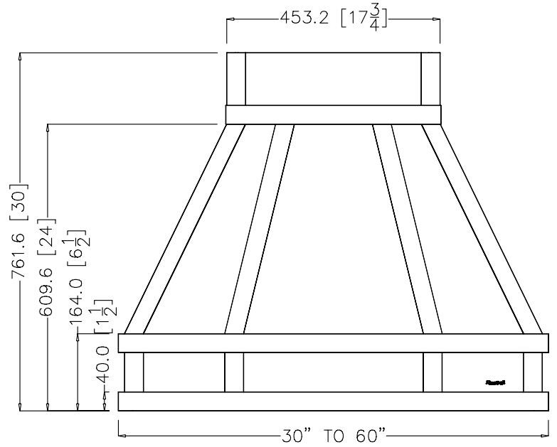
FRONT VIEW
