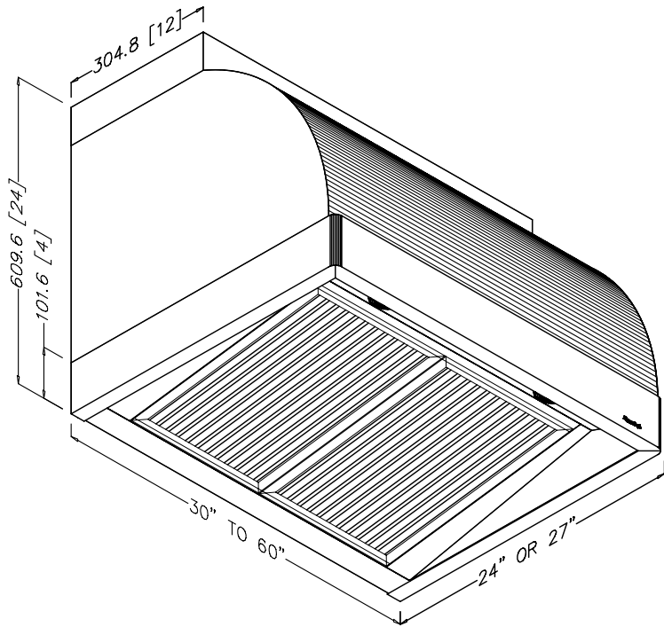
ISO VIEW
