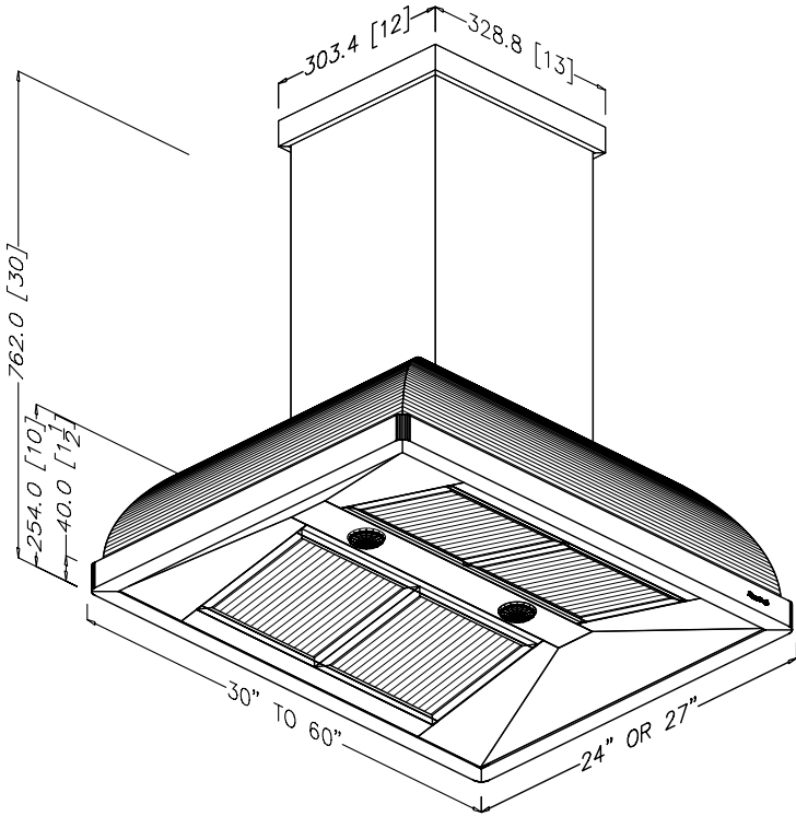
ISO VIEW
