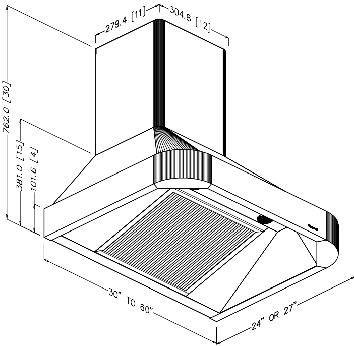
ISO VIEW
