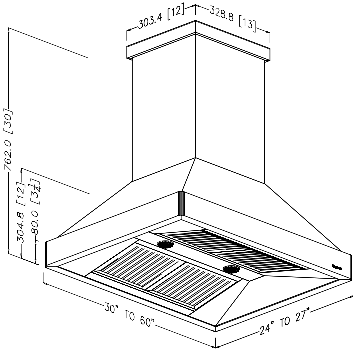
ISO VIEW
